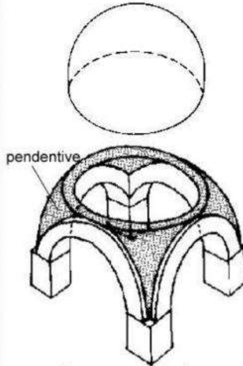
Dome supported on pendentives
