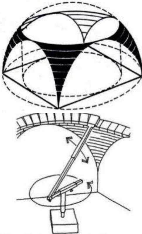
building of a dome on pendentives
